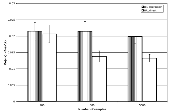
Figure 6: Comparison of sampling efficiency of best response methods in two-player first-price sealed-bid auctions.
