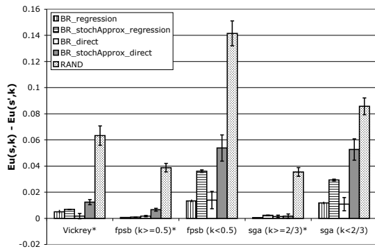
Figure 3: Comparison of best response methods in 2-player games with reserve price = 0.
